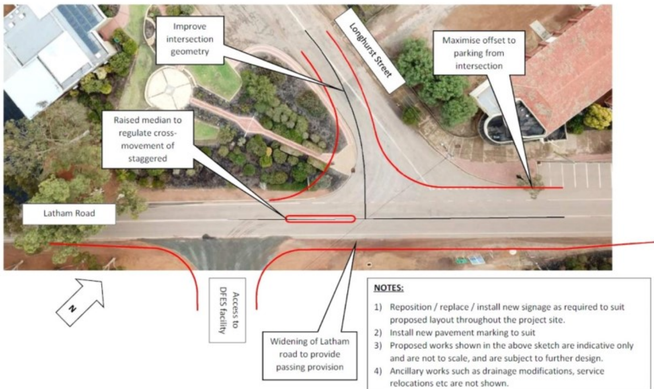
Sketch of proposed treatments to Latham Road & Longhurst Street, Naremben townsite, Shire of Naremben
